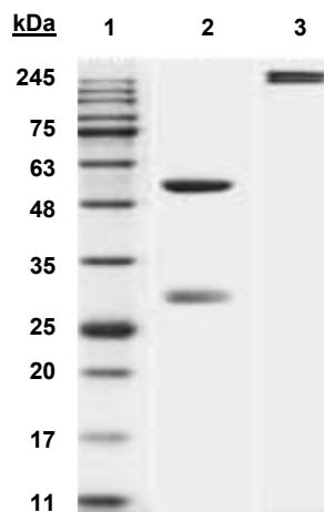
Figure 1: SDS-PAGE Analysis
