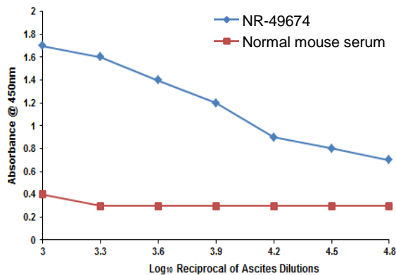
Figure 1 – ELISA
