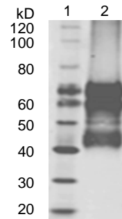
Figure 2 – Western Blot
